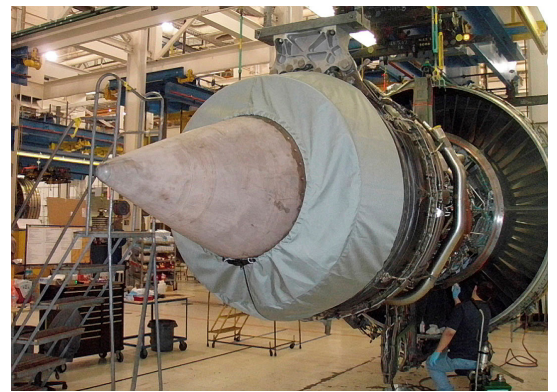
PW4077 Maintenance Exhaust ShowerCap, P/N: PW-119
