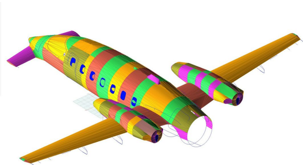
Piaggio P180 Fuselage/Canard Cover & Wing/Engine Covers (test fit covers) Piaggio P180 Fuselage, Canard, Wing & Engine Covers, 3D model
