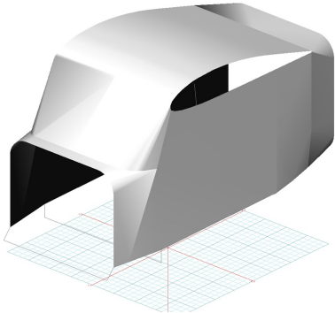
Murphy Moose Extended Canopy Cover, Engine & Prop Covers, test fit covers. Murphy Rebel Extended Canopy Cover, 3D model
