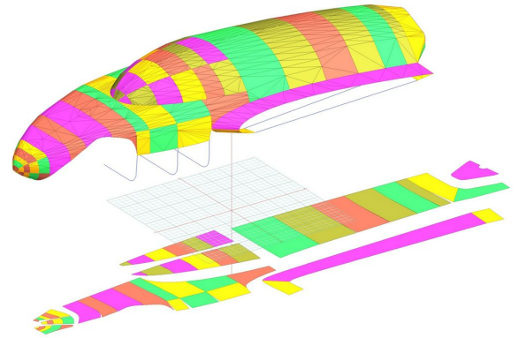
Cozy MkIV Canopy/Nose/Engine Cover, 3D model
