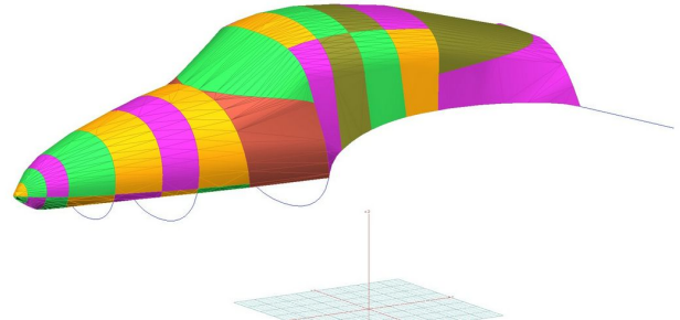
Canadair CT-114 Tutor Canopy/Nose Cover
