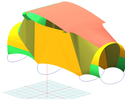
Aermacchi AM-3 Bosbok Canopy Cover (3D Model)
