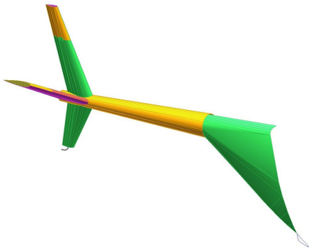
McDonnell Douglas 500C (OH-6, OH-6A, AH-6J, TH-6) Tailboom Cover (3D model)
