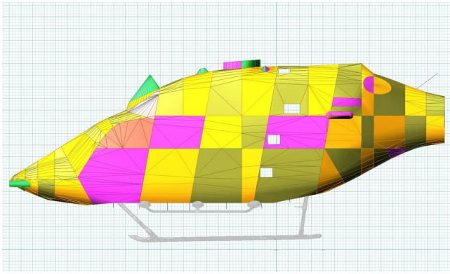
Bell 429 Main Body Cover, 3D model
